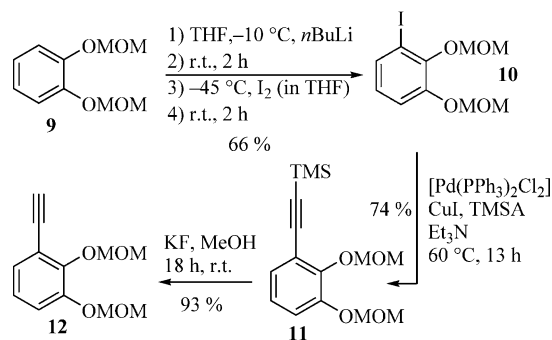
Scheme 3. Synthesis of monofunctionalized MOM-protected catechol derivatives 10–12 .
