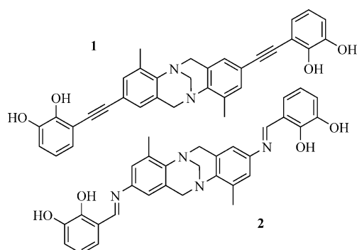
Figure 2. Bis(catechol) ligands 1 (ethynediyl bridged) and 2 (iminediyl bridged) derived from analogues of Tröger's base.
