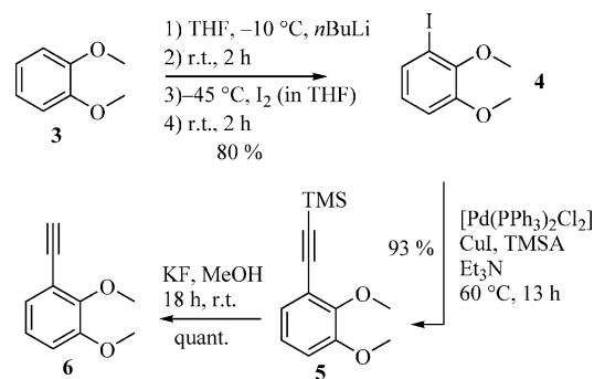
Scheme 1. Synthesis of monofunctionalized veratrol derivatives 4 – 6 .
