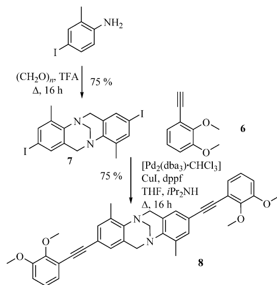
Scheme 2. Synthesis of racemic precursor 8 .
