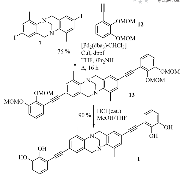
Scheme 4. Synthesis of precursor 13 and deprotection to racemic 1 .
