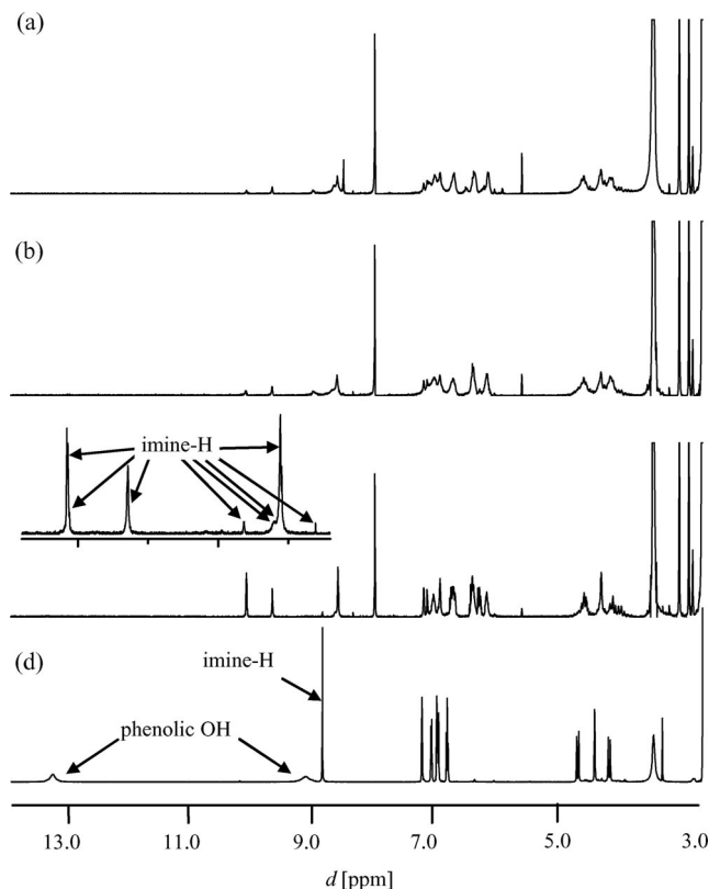
Figure 5. ^1\text{H} NMR spectroscopic complexation studies of 2 in [\text{D}_6] -DMSO: (a) \text{K}_4[\text{Ti}_2(\mathbf{2})_3] ; (b) \text{Na}_4[\text{Ti}_2(\mathbf{2})_3] ; (c) \text{Li}_4[\text{Ti}_2(\mathbf{2})_3] ; (d) 2 .
