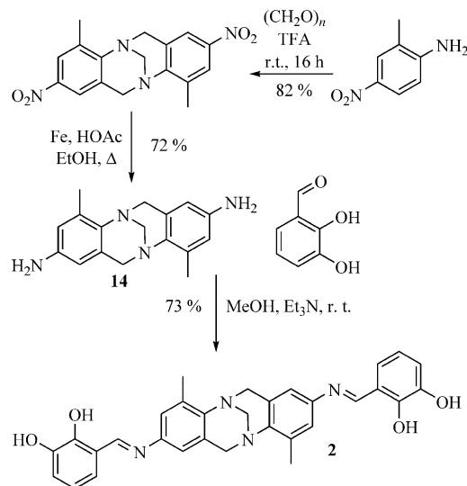
Scheme 5. Synthesis of racemic ligand 2 .
