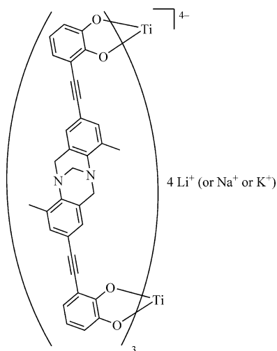
Figure 3. Schematic figure of dinuclear triple-stranded complex with \text{Ti}^{\text{IV}} derived from 1 .
