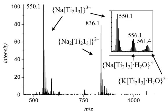
Figure 4. Negative ESI-MS of a solution of \text{Na}_4[\text{Ti}_2(\mathbf{1})_3] in MeOH/DMF.
